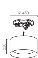
BEVEL ROUND 450
