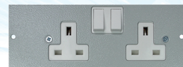
STO290/RH Right Hand Twin Switched Sockets
