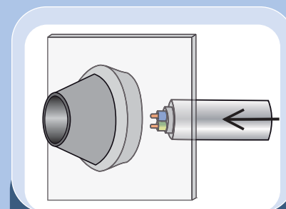
Deformable lip adapting to a wall thickness of 1 to 4 mm.
