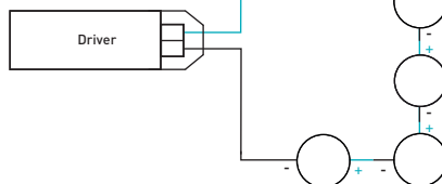
Series wiring diagram for constant current
