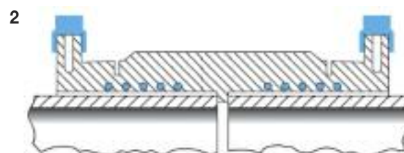
Coil energised.
