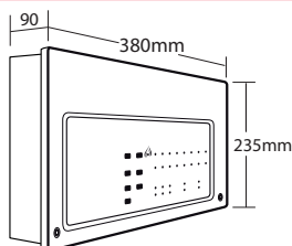
CFP 2-8 ZONE PANEL Hole required for flush mounting: W 367 x H 220 x D 75mm approx (No bezel required)
