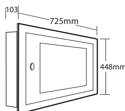
BF359/35 STAINLESS STEEL ENCLOSURE Depth of hole required for flush mounting: 93mm
