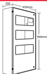
ZFP LARGE PANEL
