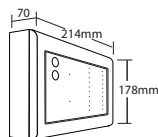
NC910/920 SURFACE CALLCONTROLLER Designed for surface mounting only
