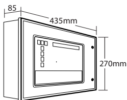
QT60I-2 CONTROLLER Hole required for flush mounting using AFP385 bezel: W 412 x H 255 x D 50 approx
