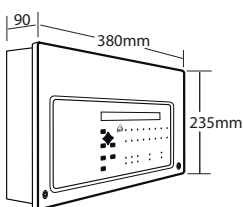
XFP 1 LOOP 16Z PANEL Hole required for flush mounting: W 367 x H 220 x D 75mm approx (No bezel required)
