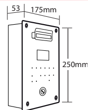
EP210F RSU Hole required for flush mounting: W 156 x H 232 x D 51mm approx (No bezel required)
