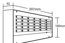
IO-30Z INDICATOR PANEL Designed for surface mounting only
