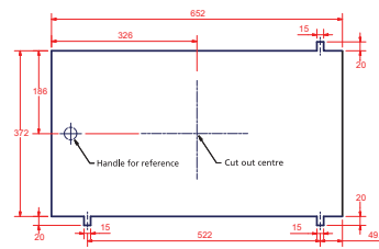
BF359/35 STAINLESS STEEL ENCLOSURE Depth of hole required for flush mounting: 93mm
