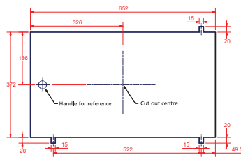
BF359/3S STAINLESS STEEL ENCLOSURE Depth of hole required for flush mounting: 93mm
