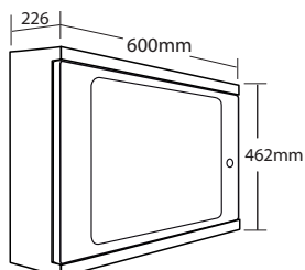
BF359/2 ENCLOSURE Hole required for flush mounting using BF359/2B bezel: W 610 x H 470 x D 185mm approx
