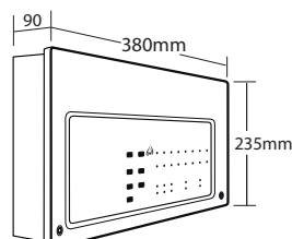
QT630 DEMENTIA CONTROLLER Hole required for flush mounting: W 367 x H 220 x D 75mm approx (No bezel required)
