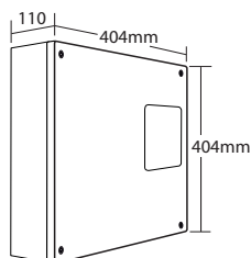
BF362-1/3/5 PSU Designed for surface mounting only
