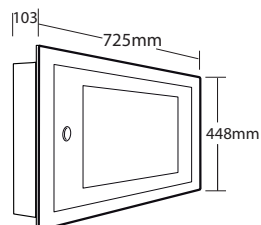
BF359/3S STAINLESS STEEL ENCLOSURE Depth of hole required for flush mounting: 93mm
