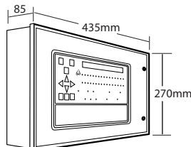
XFP 1/2 LOOP 32Z PANEL Hole required for flush mounting using AFP385 bezel: W 412 x H 255 x D 50 approx
