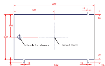
BF359/3D STAINLESS STEEL ENCLOSURE Depth of hole required for flush mounting: 183mm
