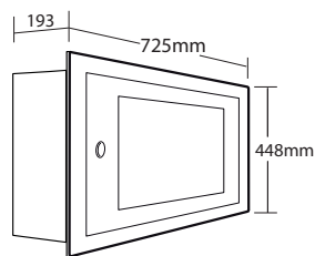
BF359/3D STAINLESS STEEL ENCLOSURE Depth of hole required for flush mounting: 183mm
