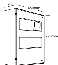
ZFP MEDIUM PANEL
