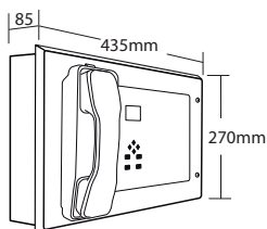
ECU-4/8 CONTROLLER Hole required for flush mounting using AFP385 bezel: W 412 x H 255 x D 50 approx
