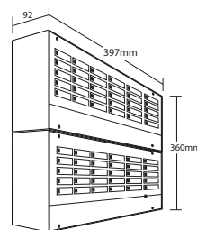
40-60Z INDICATOR PANEL Designed for surface mounting only
