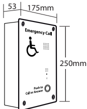
EVC302F OUTSTATION Hole required for flush mounting: W 156 x H 232 x D 51mm approx (No bezel required)
