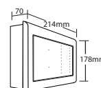
ZREPIF Hole required for flush mounting: W 176 x H 162 x D 55mm approx (No bezel required)
