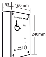
EVC302S OUTSTATION Designed for surface mounting only
