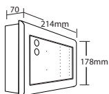
NC910/920 FLUSH CALLCONTROLLER Hole required for flush mounting: W 176 x H 162 x D 55mm approx (No bezel required)
