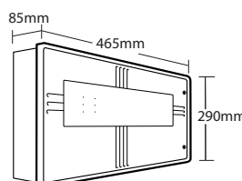
BF361-3/5 PSU Hole required for flush mounting: W 440 x H 277 x D 40mm approx
