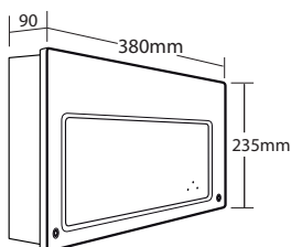
BF360-12/24 PSU Hole required for flush mounting: W 367 x H 220 x D 75mm approx (No bezel required)
