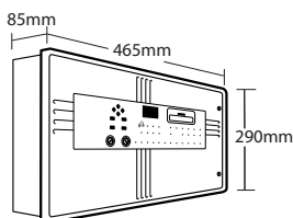
EP203 PANEL Hole required for flush mounting: W 440 x H 277 x D 40mm approx
